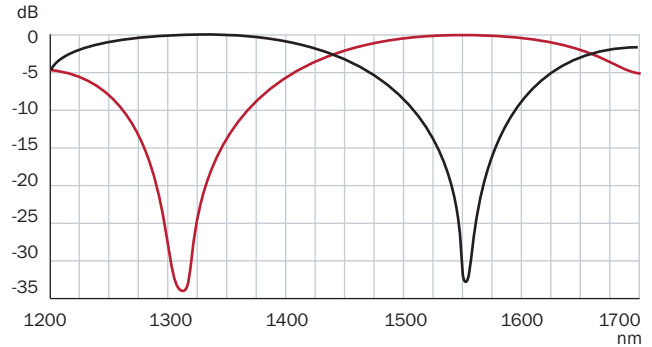
Wavelength dependence of WWDWM with central wavelengths 1310 nm and 1550 nm
